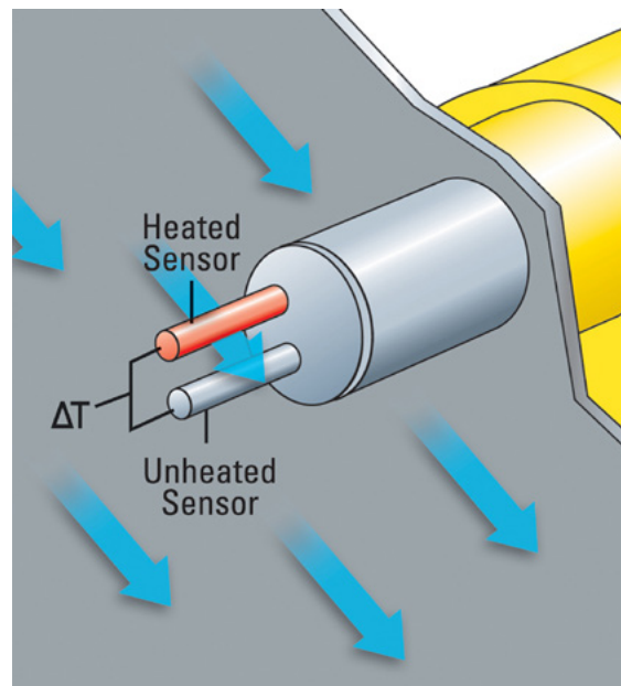
Figure 3: Thermal dispersion technology principle of operation
